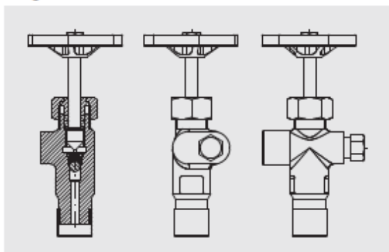
Model LGV-33 Forged valve with handwheel
