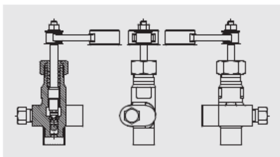
Model LGV-38 Forged valve with quick closing lever
