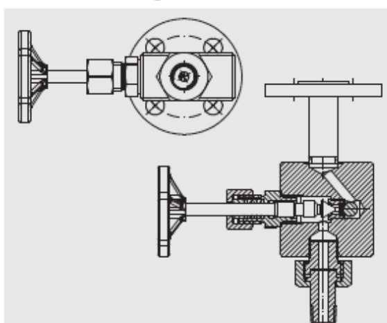
Model LGV-51, straight valve with handwheel
