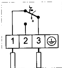
Abb. 11. ABC*...-205
