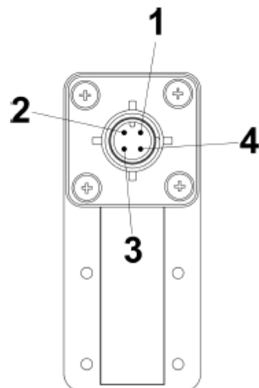
Fig. 17: Pin-assignment, socket M12x1 Form 30x70)
