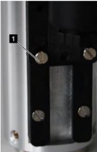
Fig. 33: Loosen set screws
