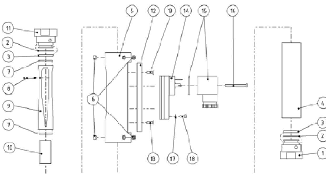
Fig. 66: Spare parts drawing
