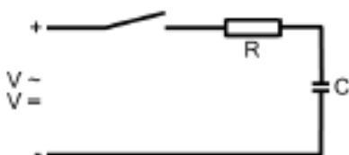
Fig. 30: Protective measure against capacitive loads
