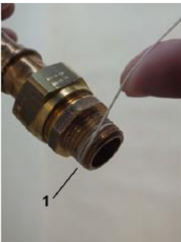
Fig. 9: Apply sealing thread
