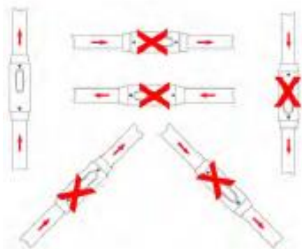
Fig. 5: Installation position/direction of flow
