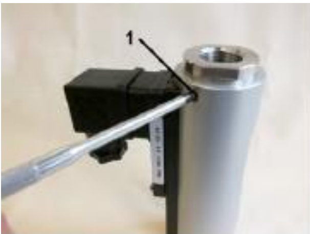
Fig. 36: Loosen screws
